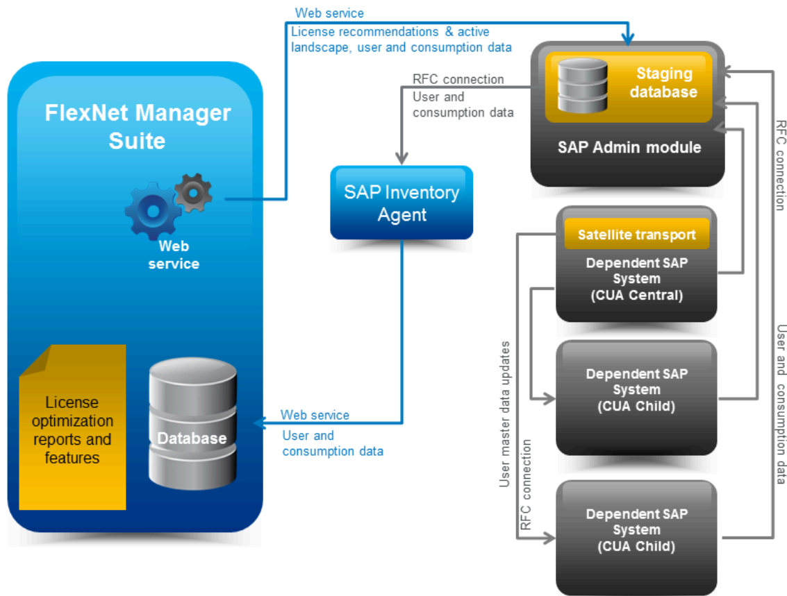
Figure 5: Data flow from FlexNet Manager Suite to the SAP systems when using CUA
