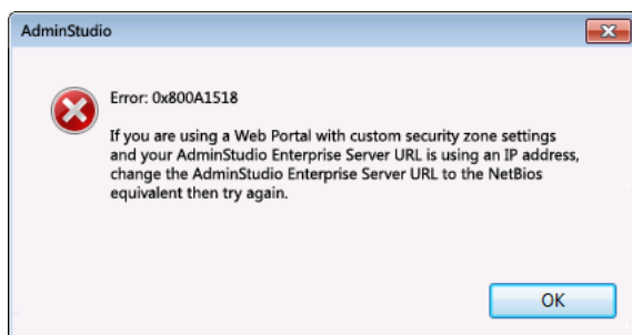
Figure 7-10: Error 0x800A1518
