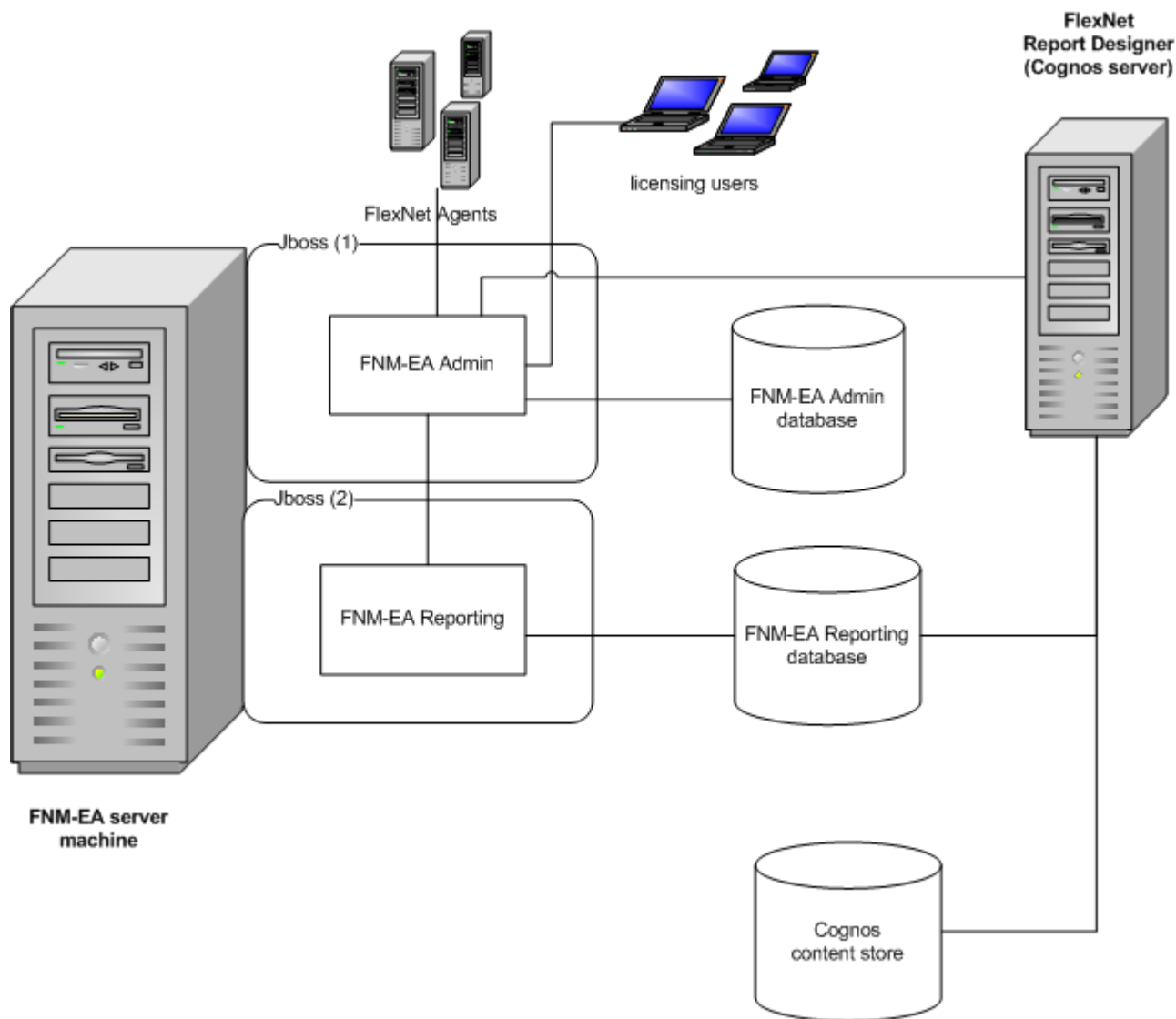
Figure 2-2: Basic FlexNet Manager for Engineering Applications 15.2 deployment with FlexNet Report Designer (Cognos)
