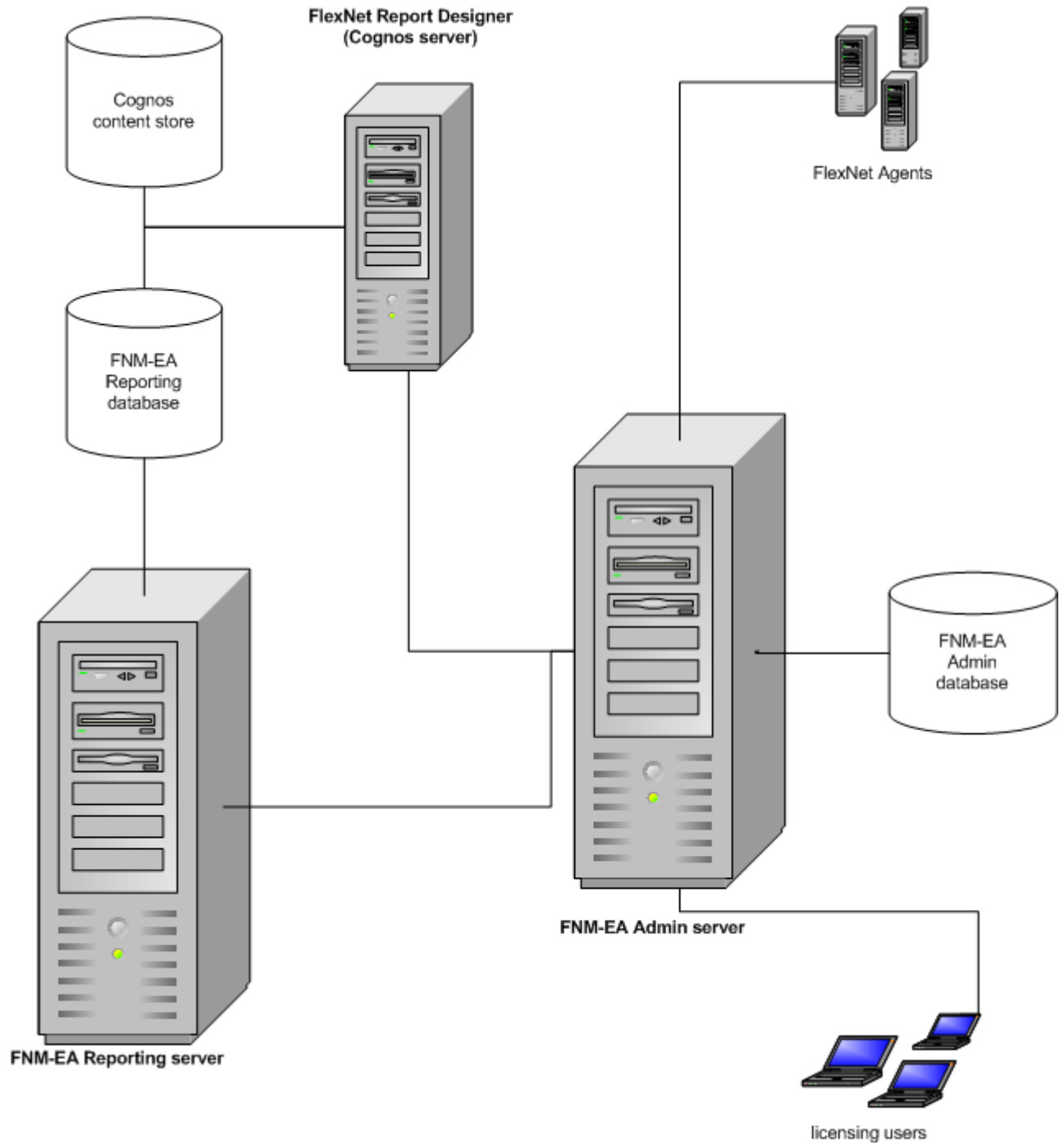
Figure 1-1: Recommended deployment design, using separate server machines for FlexNet Manager for Engineering Applications Reporting and Admin.
