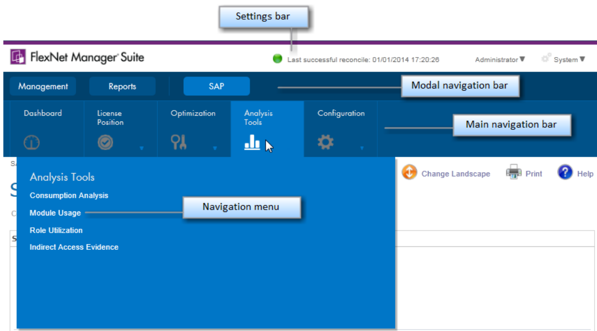
Figure 5-1: Navigation elements of a page in FlexNet Manager Suite
