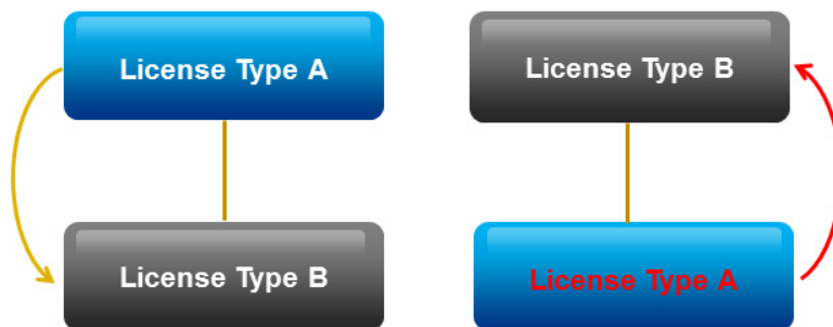
Figure 6-2: Example for a cycle in the license-type hierarchy. To remove the cycle, the sub-license type A (red) needs to be removed from license type B.
