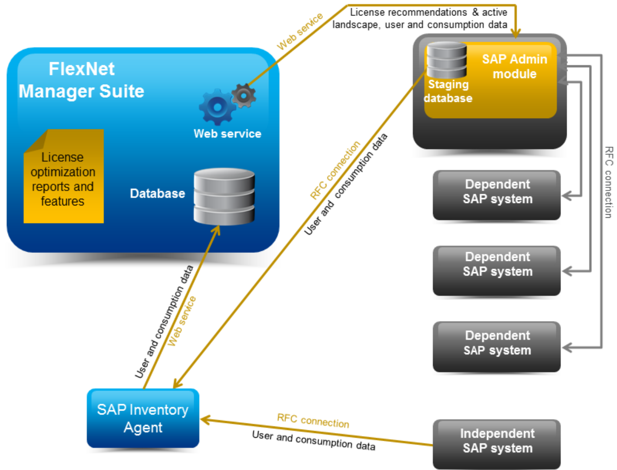
Figure 1: Data flow between the components in an on-premise implementation
