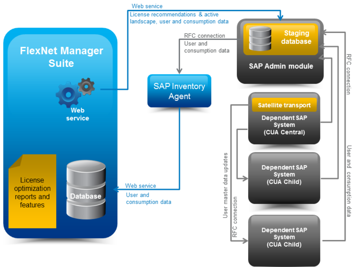
Figure 2: Data flow from FlexNet Manager Suite to the SAP systems when using CUA
