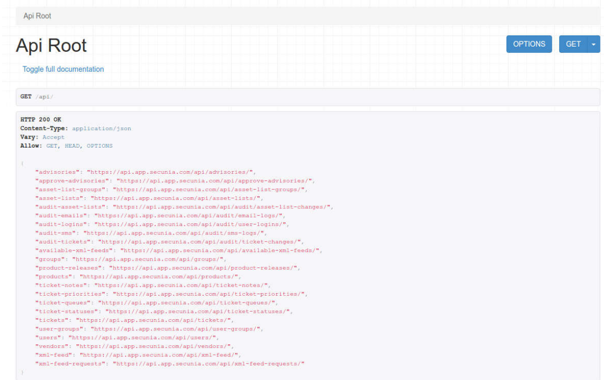
Figure 2-1: API Explorer Page Example
