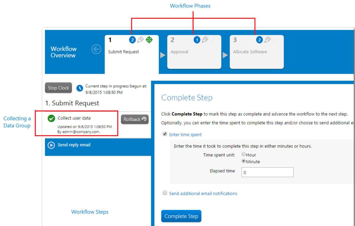
Figure 4-4: The Elements of a Workflow Template
