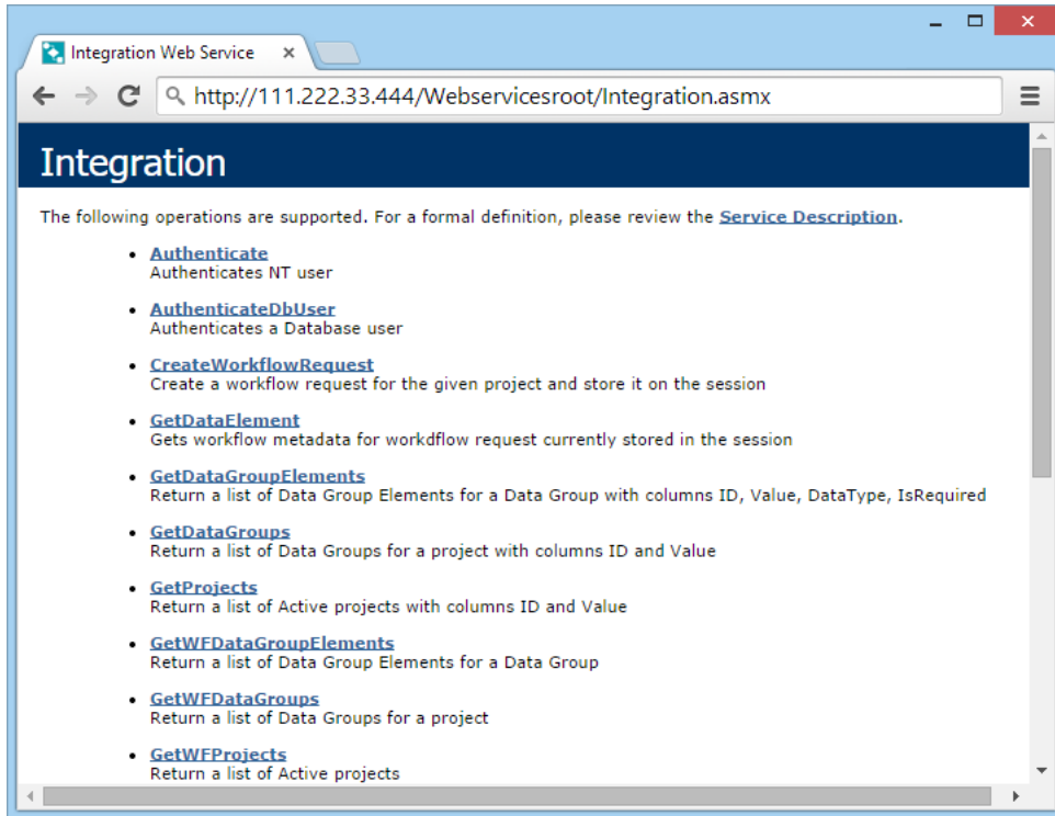
Figure 6-88: Integration Web Services Page
