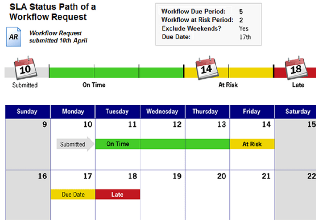
Figure 4-17: Example SLA Status Path for a Workflow Request
