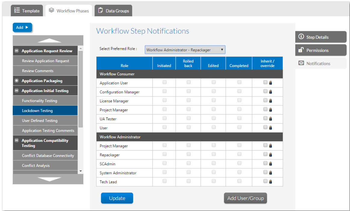
Figure 6-73: Notification Tab of Workflow Phase Details View of the Template Details Page
