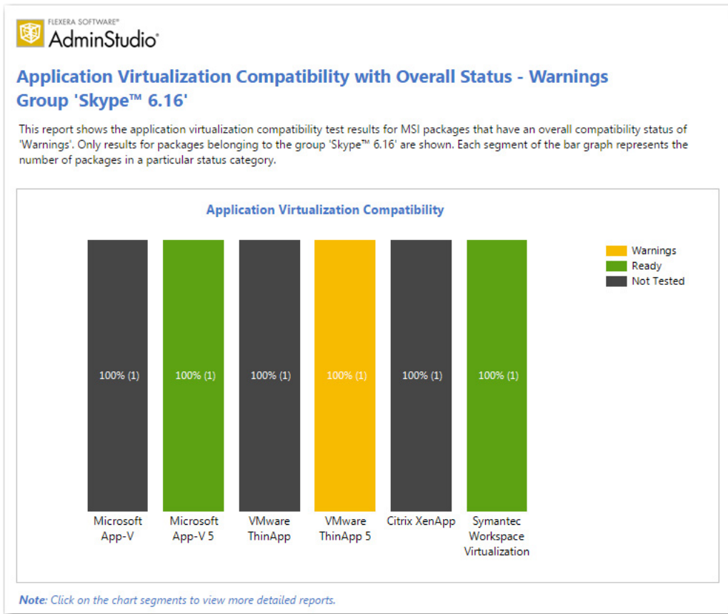
Figure 4-36: AdminStudio Report: Drill Down Report for Selected Package
