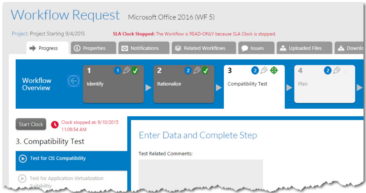
Figure 4-19: Workflow With Stopped SLA Clock
