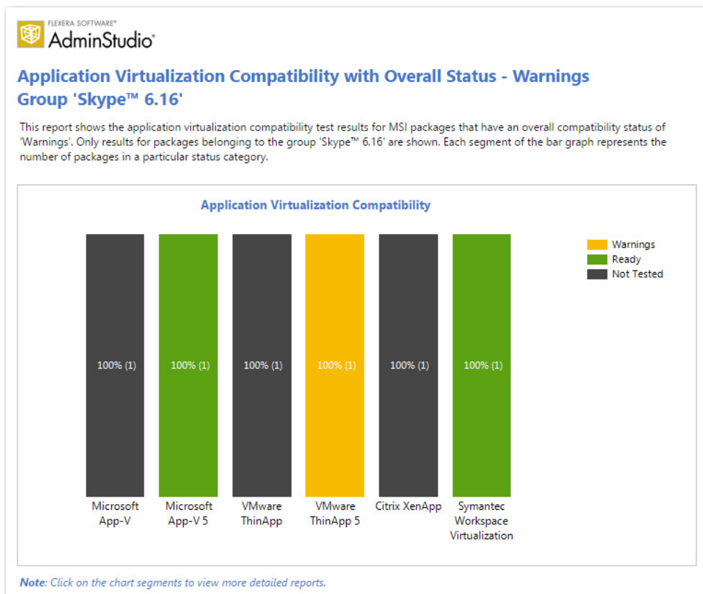
Figure 4-42: AdminStudio Report: Drill Down Report for Selected Package
