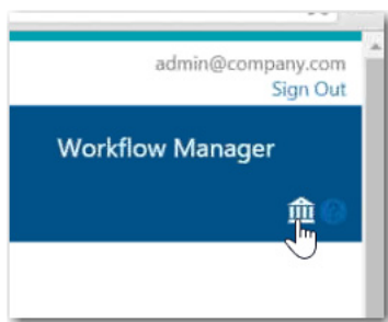
Figure 4-12: References Icon
