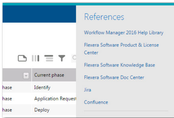
Figure 4-13: References Panel
