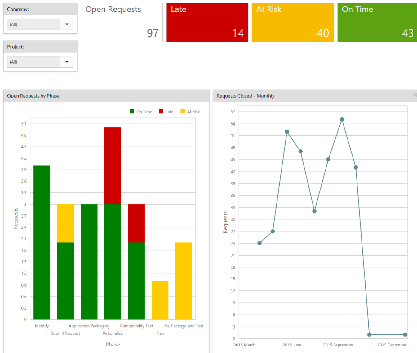
Figure 4-7: Dashboard Report
